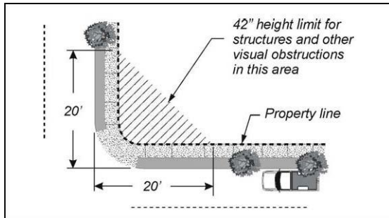
Required Traffic Safety Visibility Area
